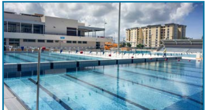
Martinique Le Lamentin, France: Movable floor and hinged bulkhead
